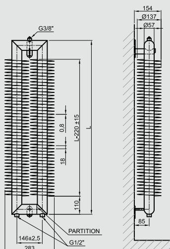
RAT2 57×2,5×137 VERTICAL
