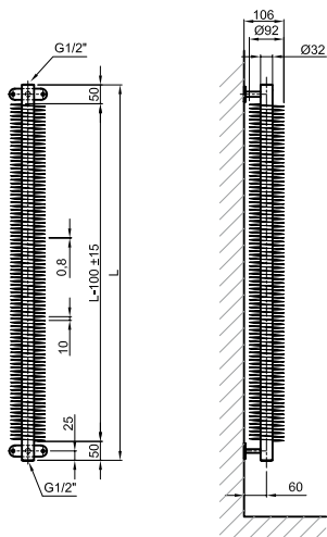
RA1 32×2×92 VERTICAL
