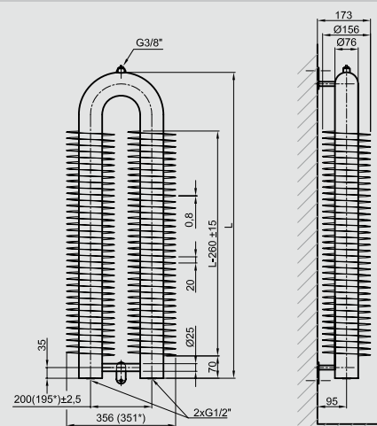
RA02 76×2,5×156 VERTICAL
