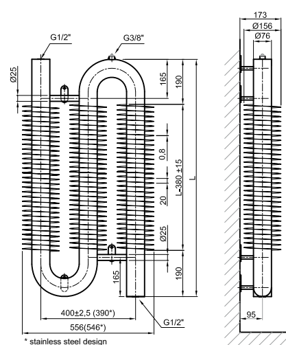
RA03 76×2,5×156 VERTICAL RIGHT
