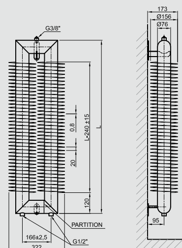
RAT2 76×2,5×156 VERTICAL
