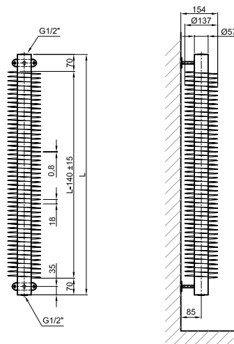
RA1 57×2,5×137 VERTICAL
