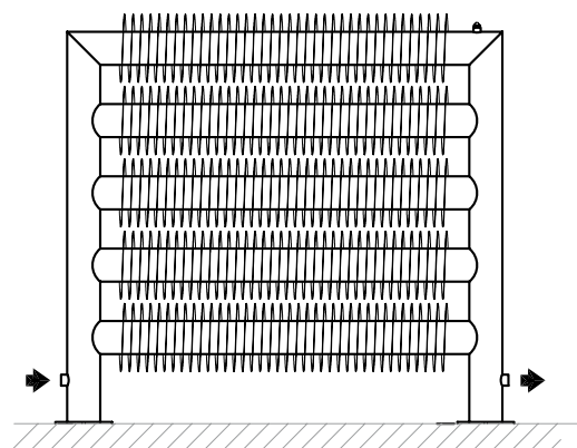
RAT5 76/156 SELF-STANDING
