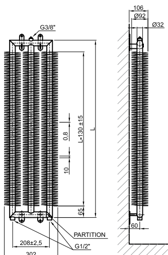
RAT3 32×2×92 VERTICAL
