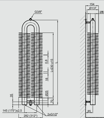
RA02 57×2,5×137 VERTICAL
