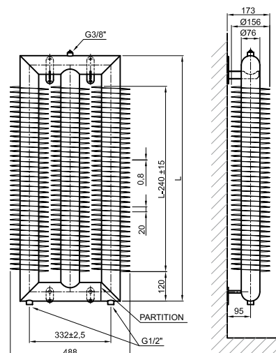
RAT3 76×2,5×156 VERTICAL
