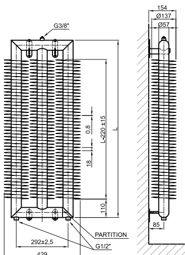
RAT3 57×2,5×137 VERTICAL
