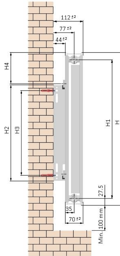
L Console mounting (long side 45 mm)
