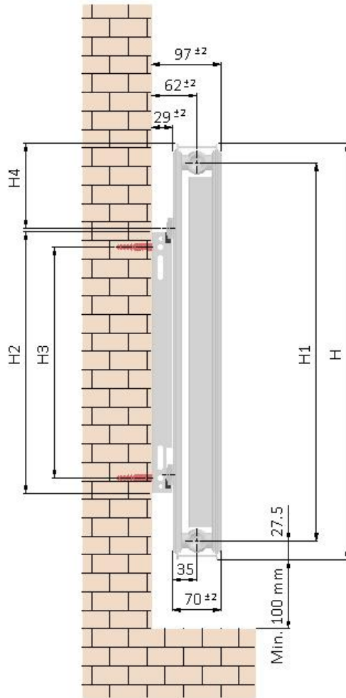
L Console mounting (short side 30 mm)
