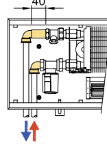
PR40 – extension piece 40 mm, 2×elbow 90° All other models FRT, FRK, except for the ones stated with PR50
