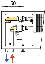
PR50 extension piece 50 mm, 2×elbow 90° Suitable for models: 0065 0175, 0065 0200, 0065 0250 0065 0300, 0080 0250, 0080 0300, 0080 0425
